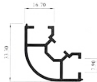
5119 (0.542 Kg./M.) SC Half Round Section
