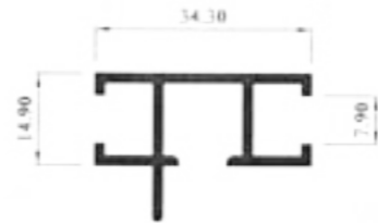
5124 (0.410 Kg./M.) SC Small Button
